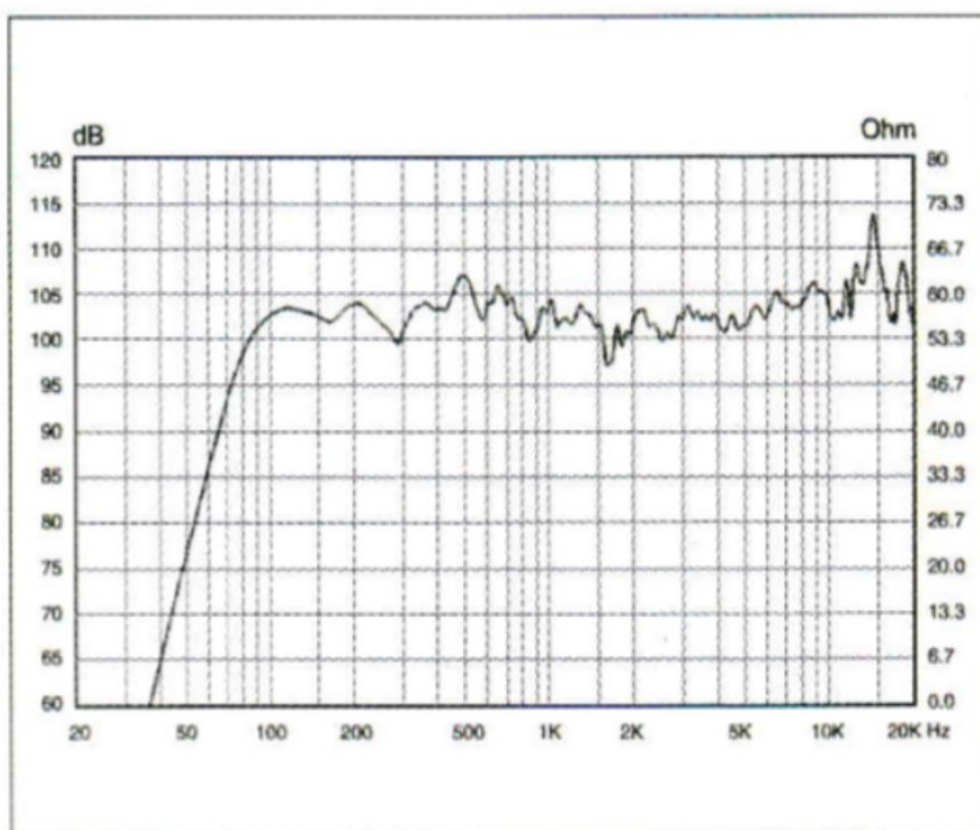
Frequency response curve
