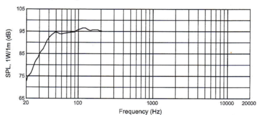
Frequency Response
